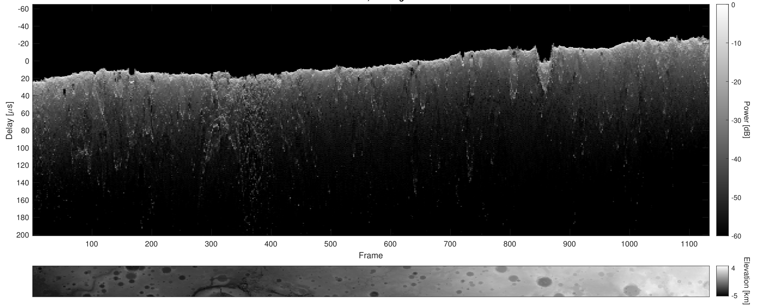
Orbit 21728, Cluttergram
