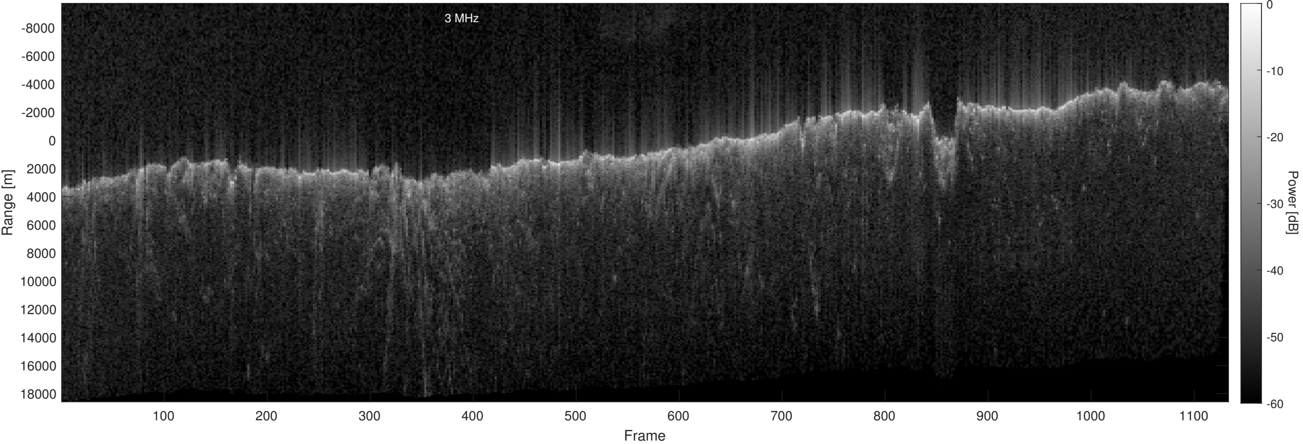
Orbit 21728, Optimized, No Window, Depth-Corrected, Channel 2
