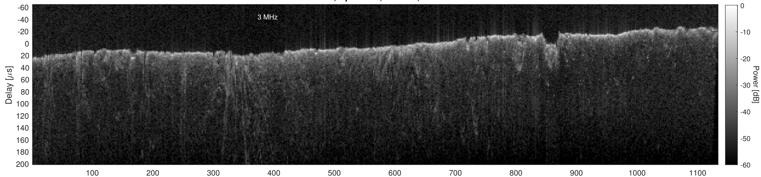
Orbit 21728, Cluttergram
