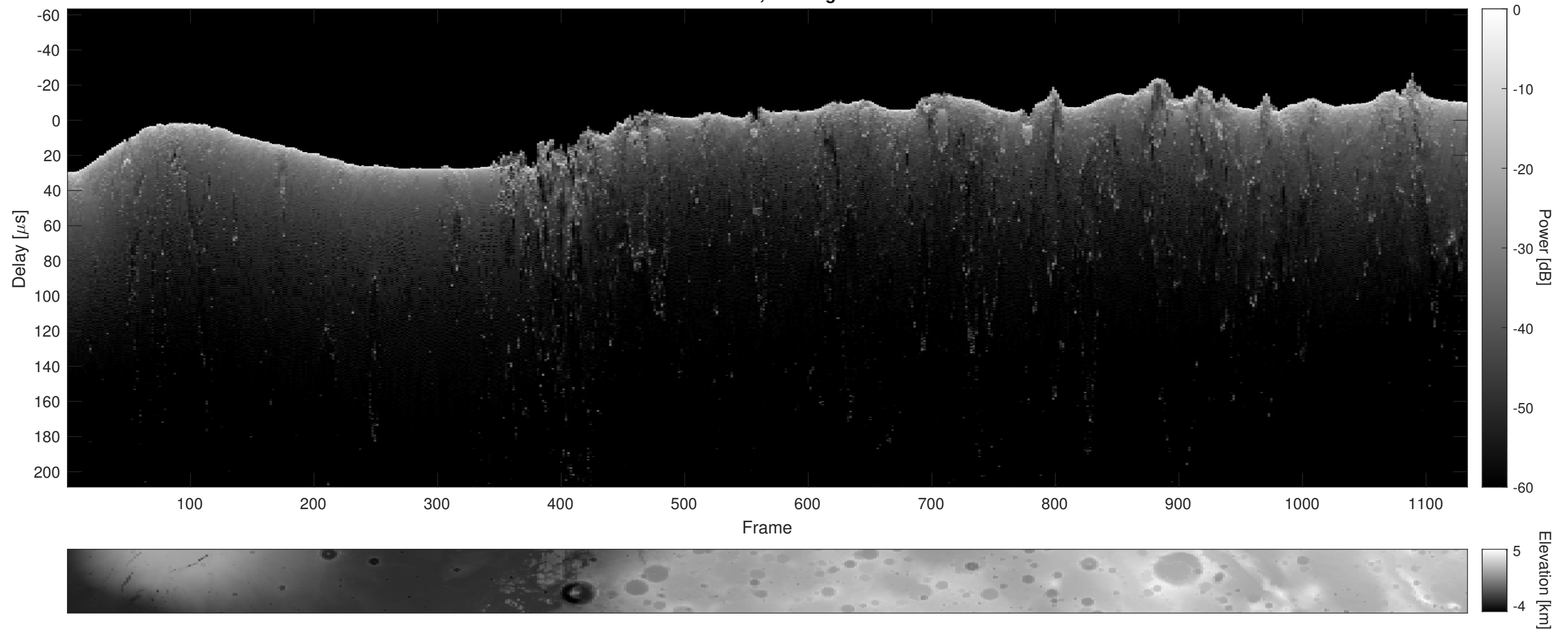
Orbit 21730, Cluttergram
