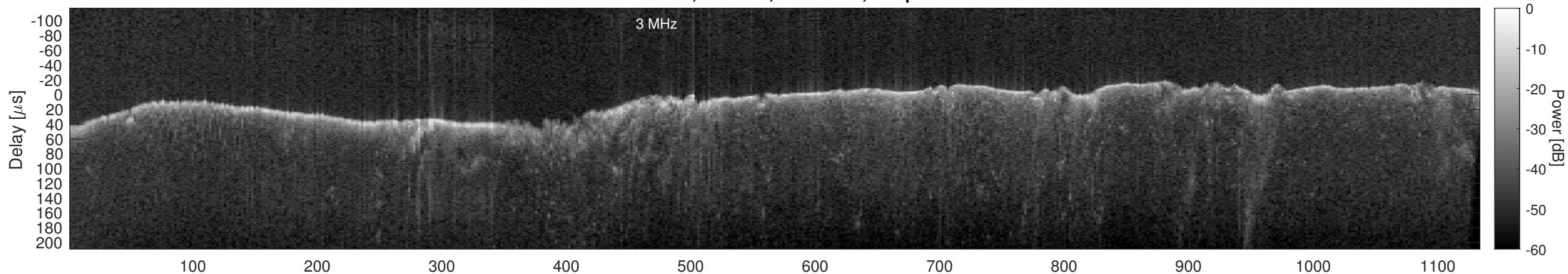
Orbit 21730, Window, Channel 2, Optimized
