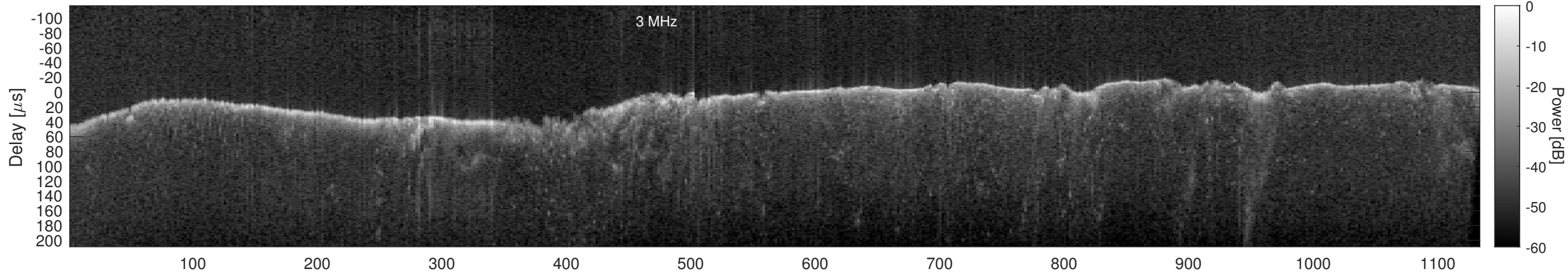
Orbit 21730, Window, Channel 2, Chapman
