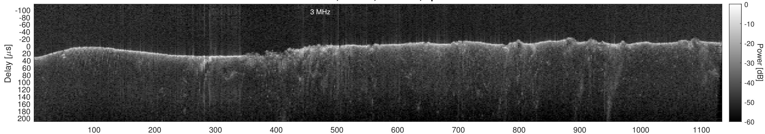
Orbit 21730, Cluttergram
