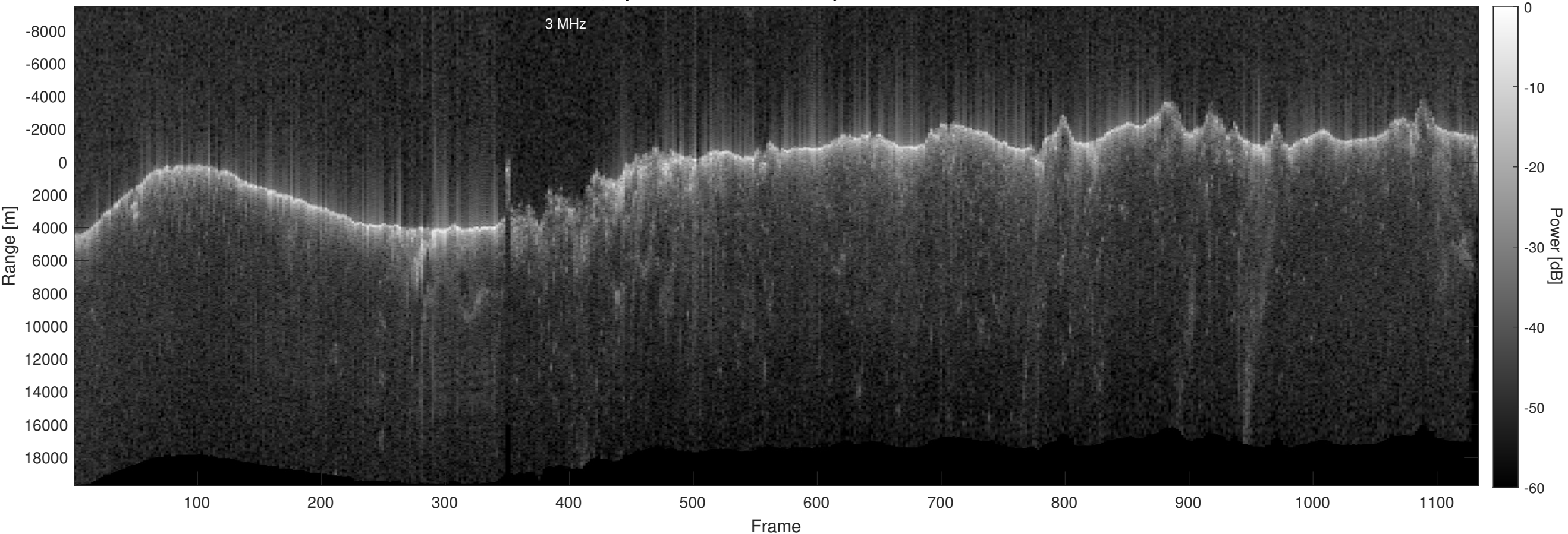
Orbit 21730, Optimized, No Window, Depth-Corrected, Channel 2
