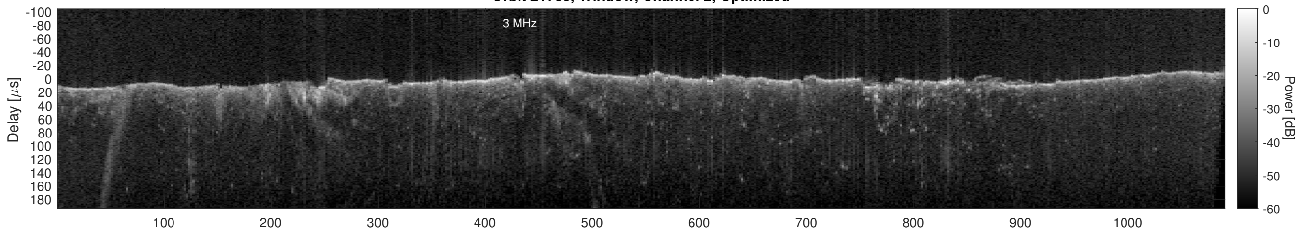
Orbit 21738, Cluttergram
