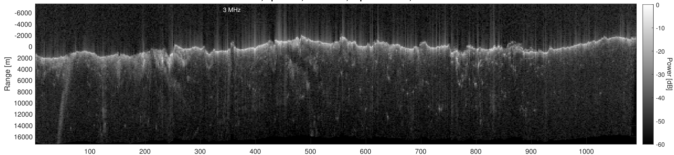
Orbit 21738, Depth-Corrected Cluttergram
