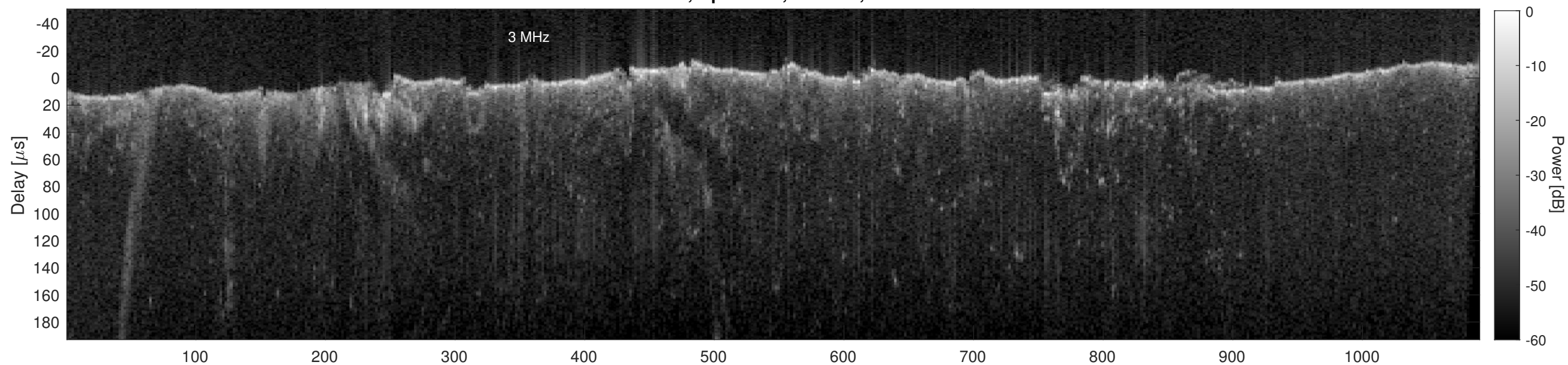
Orbit 21738, Cluttergram
