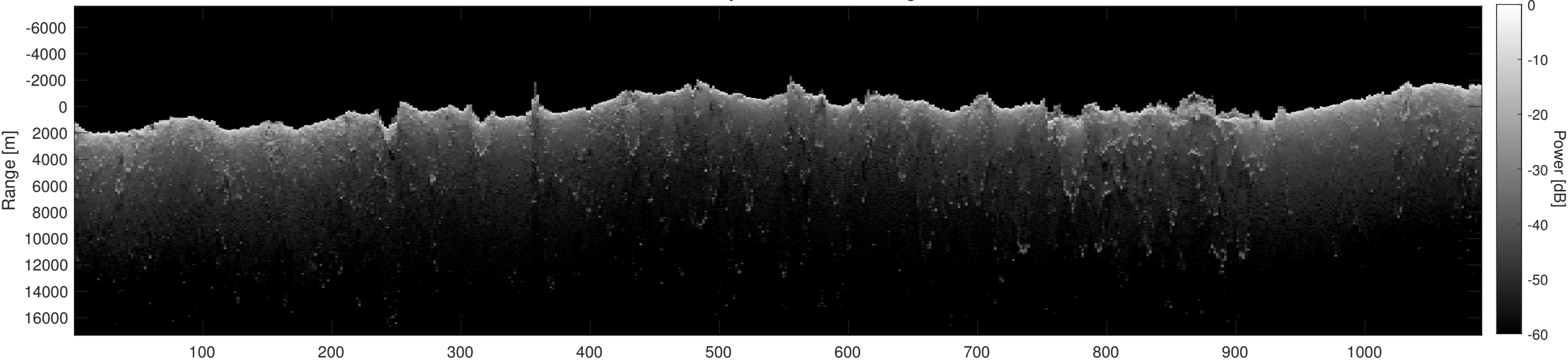
Orbit 21738, Depth-Corrected Cluttergram
