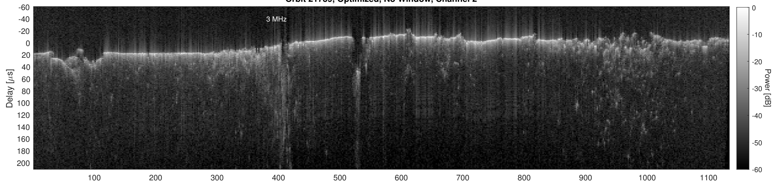
Orbit 21739, Cluttergram
