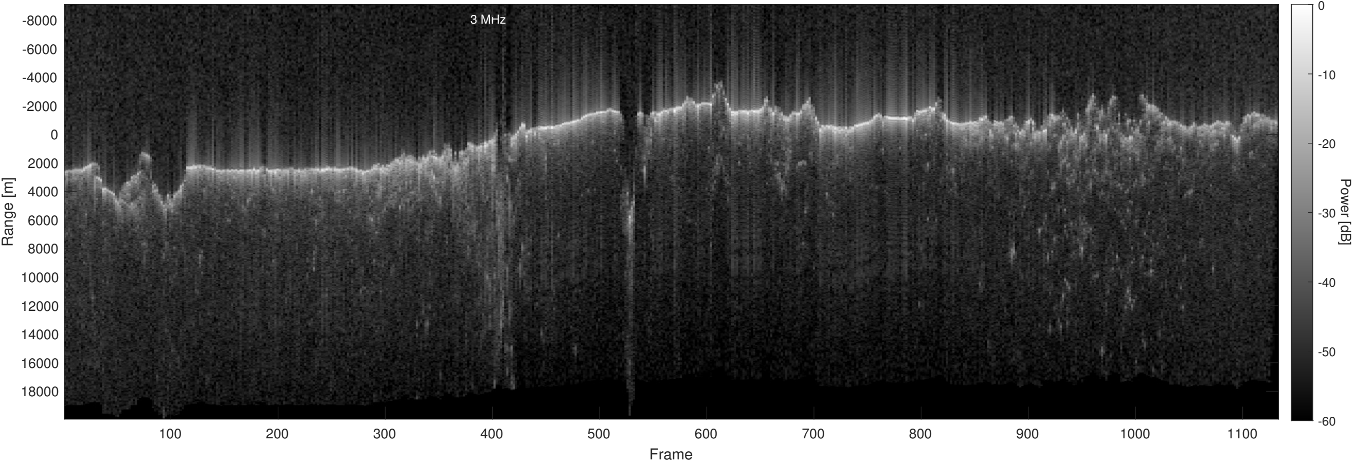
Orbit 21739, Optimized, No Window, Depth-Corrected, Channel 2
