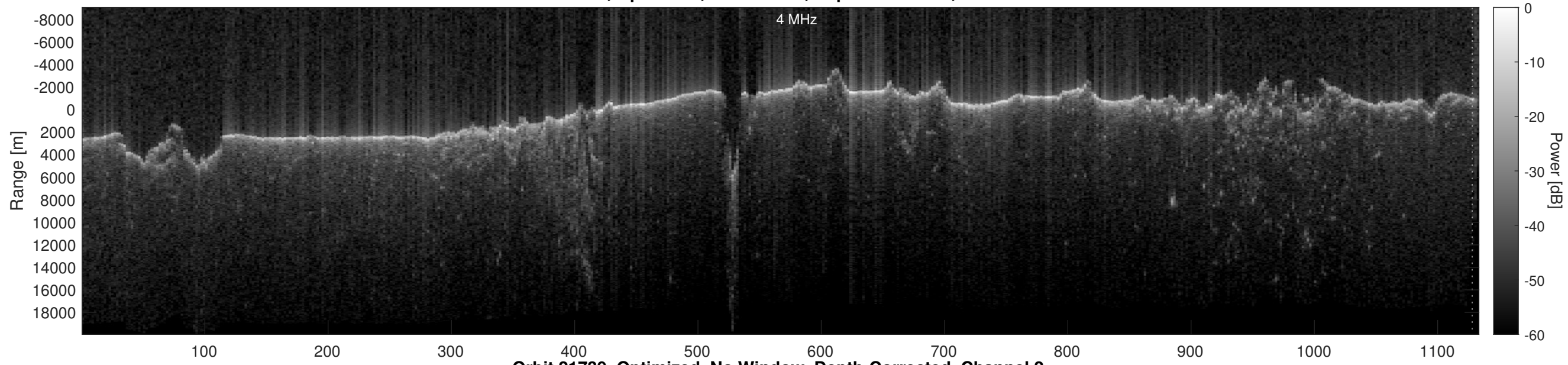
Orbit 21739, Optimized, No Window, Depth-Corrected, Channel 2
