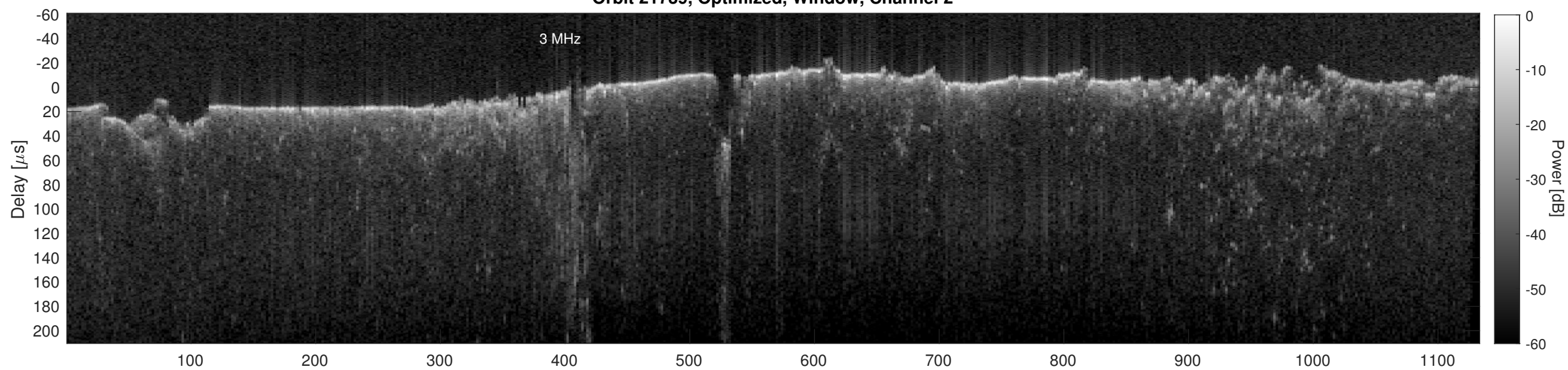
Orbit 21739, Cluttergram
