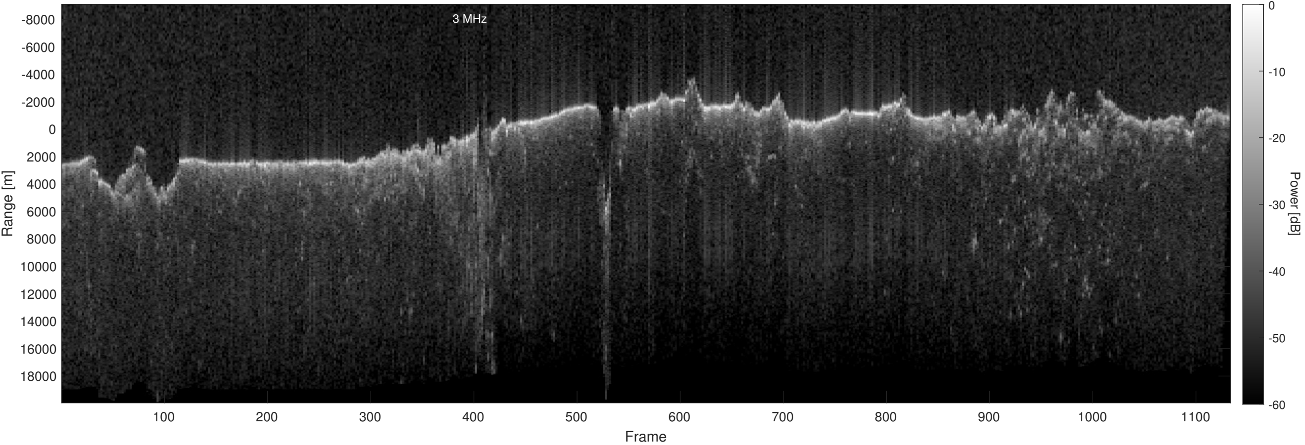
Orbit 21739, Optimized, Window, Depth-Corrected, Channel 2
