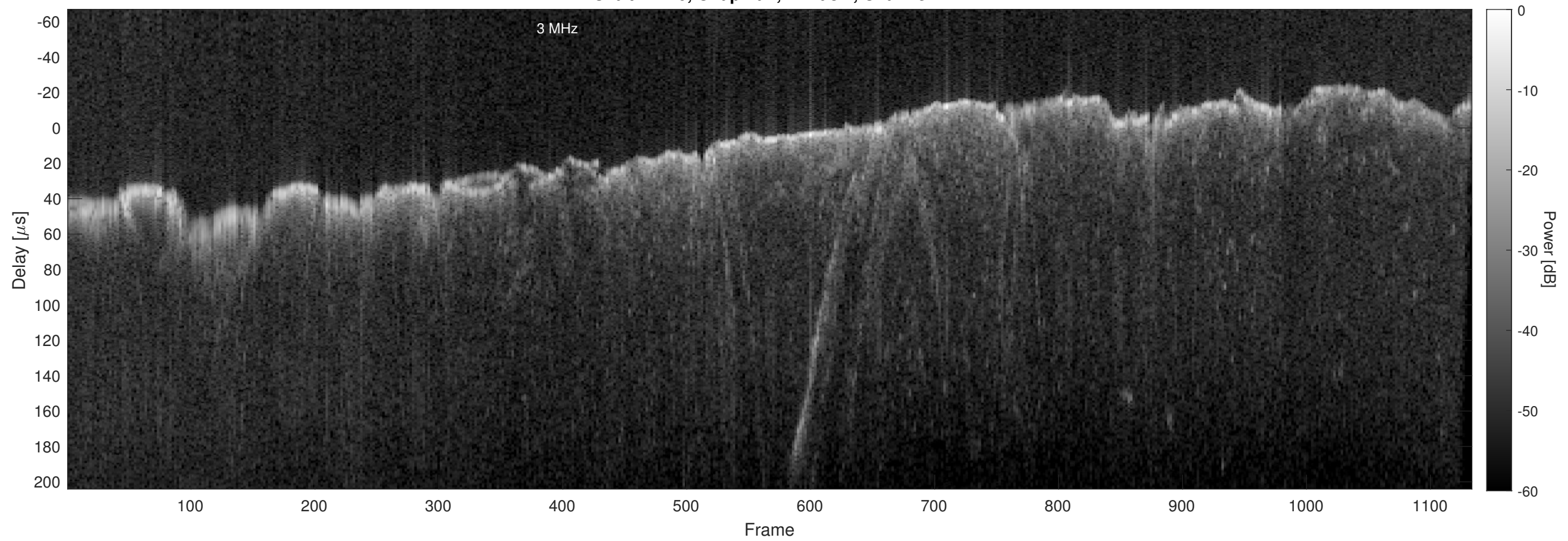
Orbit 21740, Chapman, Window, Channel 2
