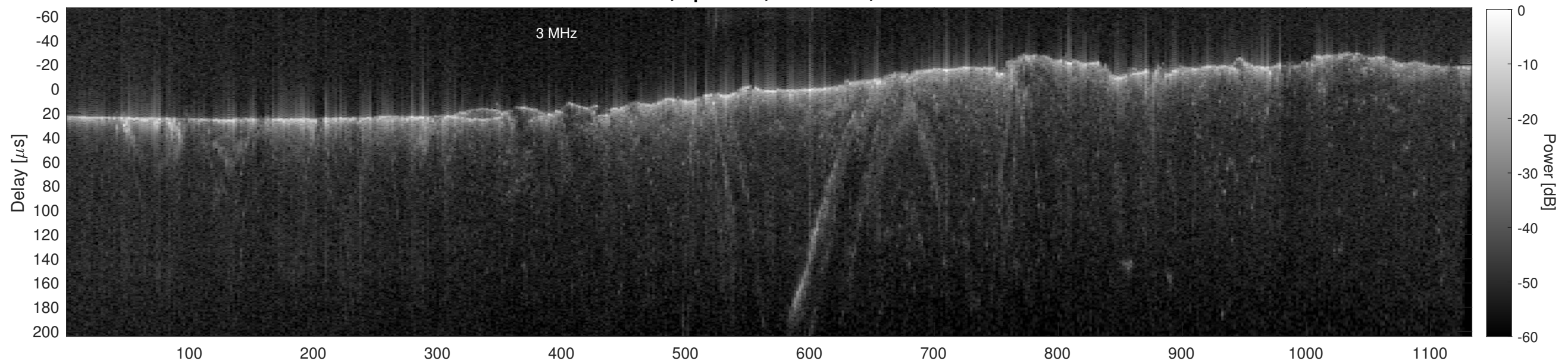
Orbit 21740, Cluttergram
