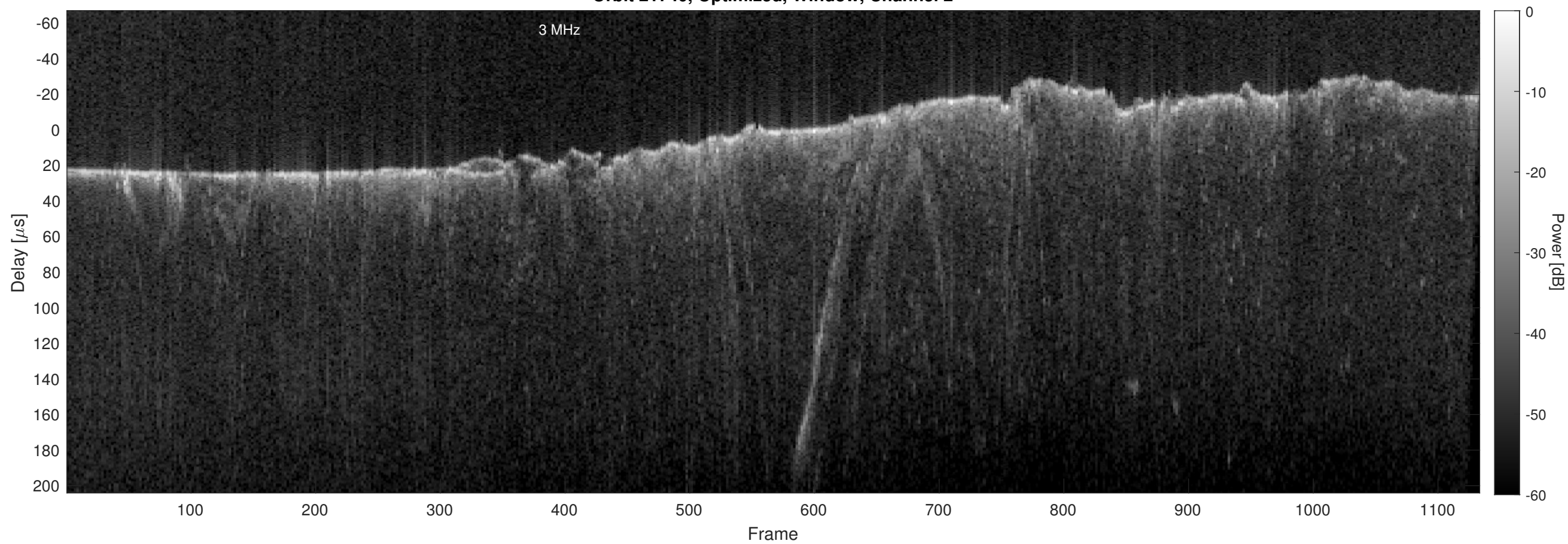
Orbit 21740, Optimized, Window, Channel 2
