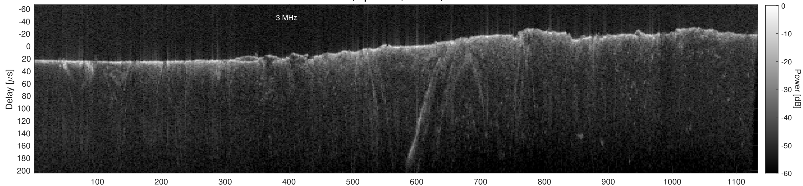
Orbit 21740, Cluttergram
