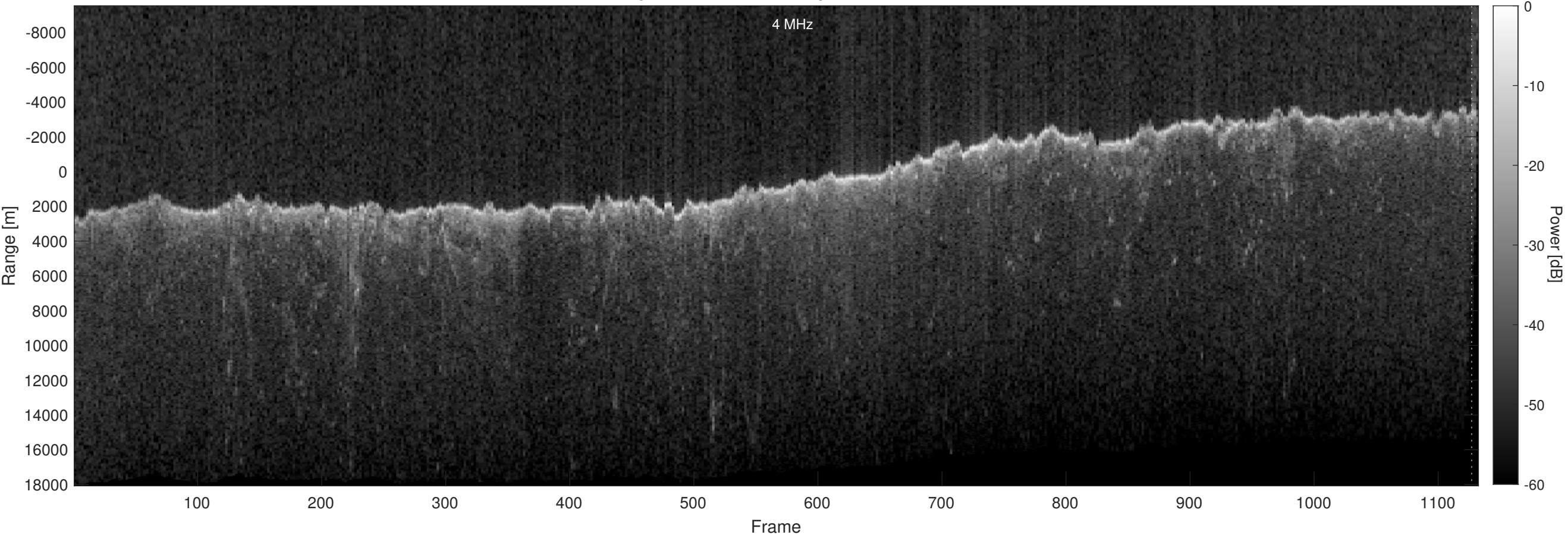
Orbit 21742, Optimized, Window, Depth-Corrected, Channel 2
