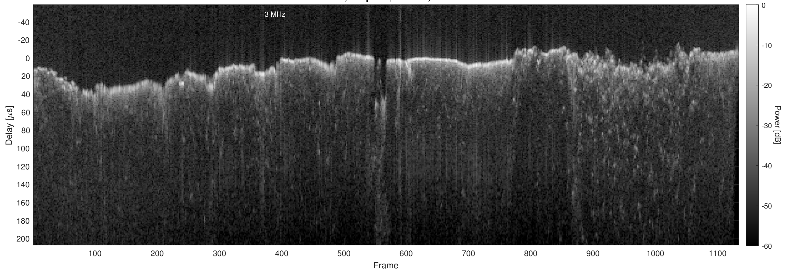
Orbit 21746, Chapman, Window, Channel 2
