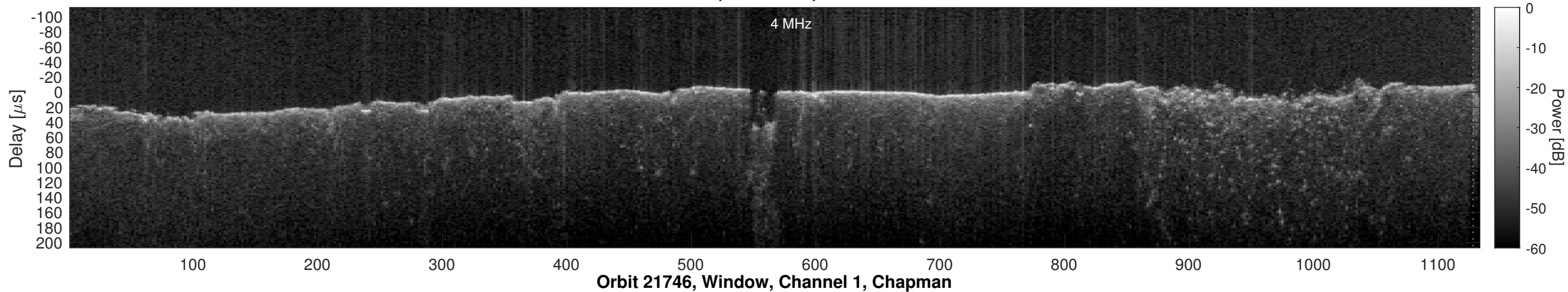
Orbit 21746, Channel 1, Uncorrected
