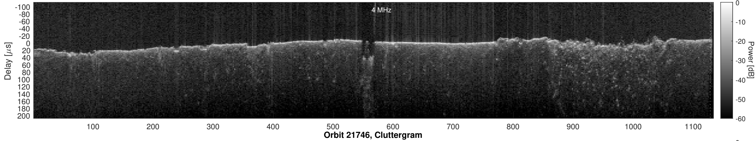
Orbit 21746, Window, Channel 1, Optimized
