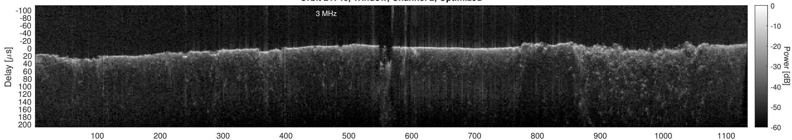
Orbit 21746, Cluttergram
