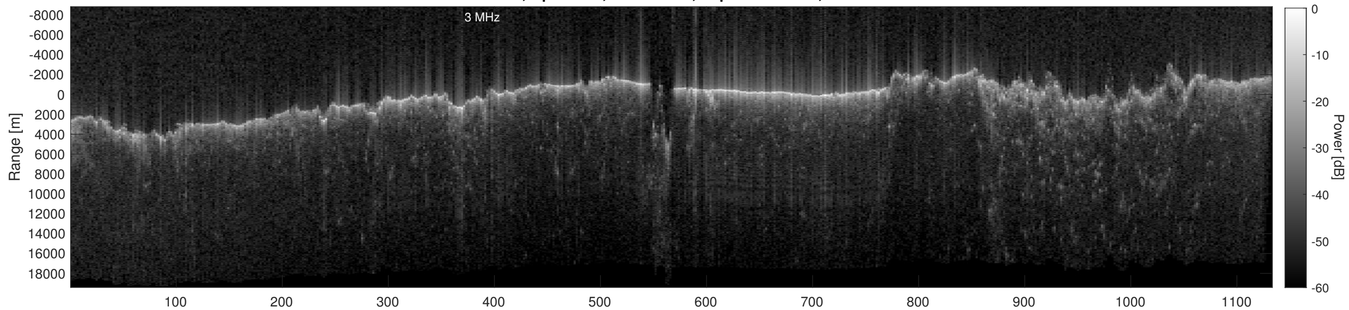
Orbit 21746, Depth-Corrected Cluttergram
