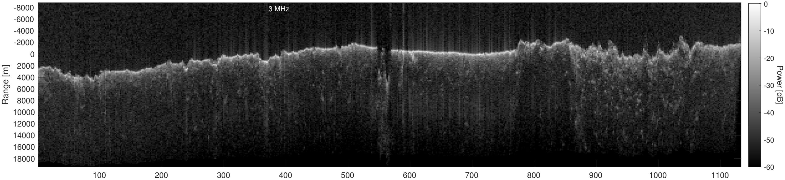
Orbit 21746, Depth-Corrected Cluttergram
