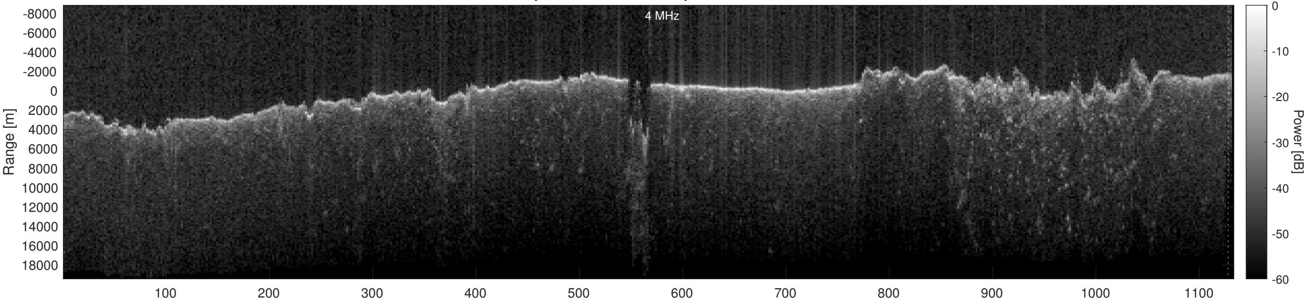
Orbit 21746, Optimized, Window, Depth-Corrected, Channel 2
