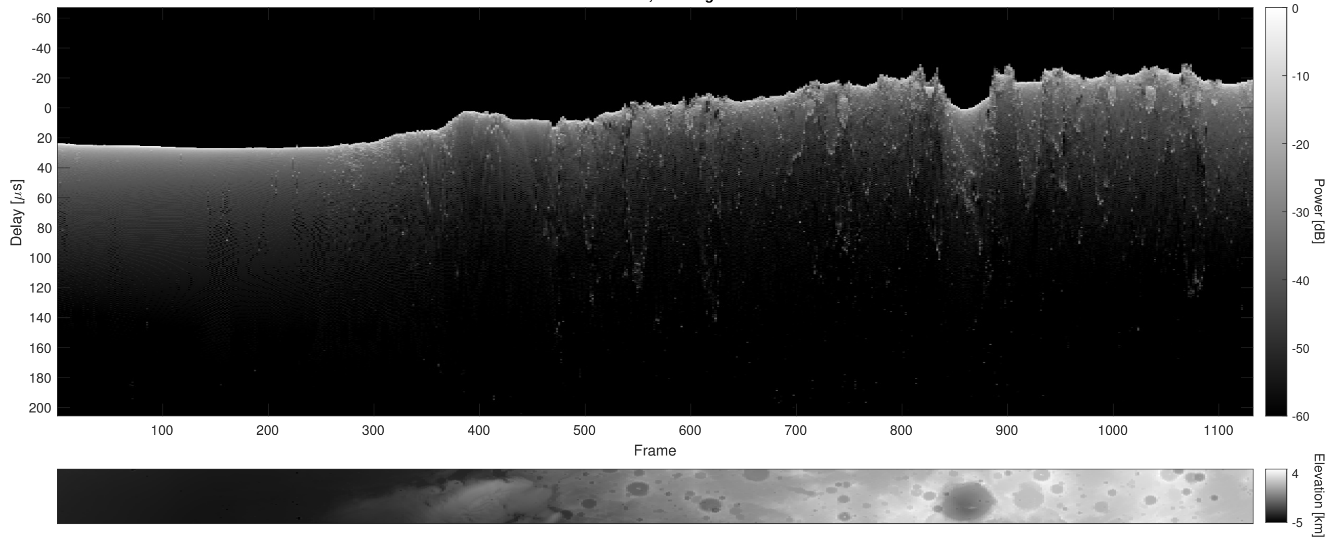
Orbit 21747, Cluttergram
