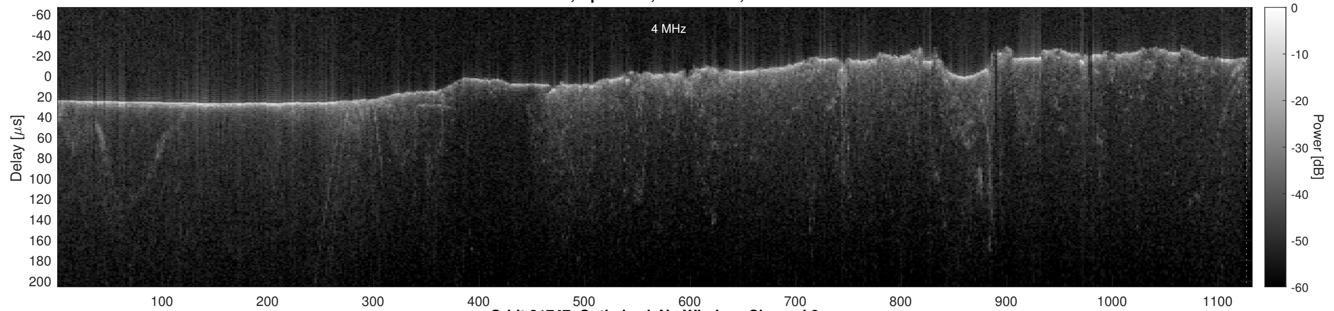
Orbit 21747, Optimized, No Window, Channel 2
