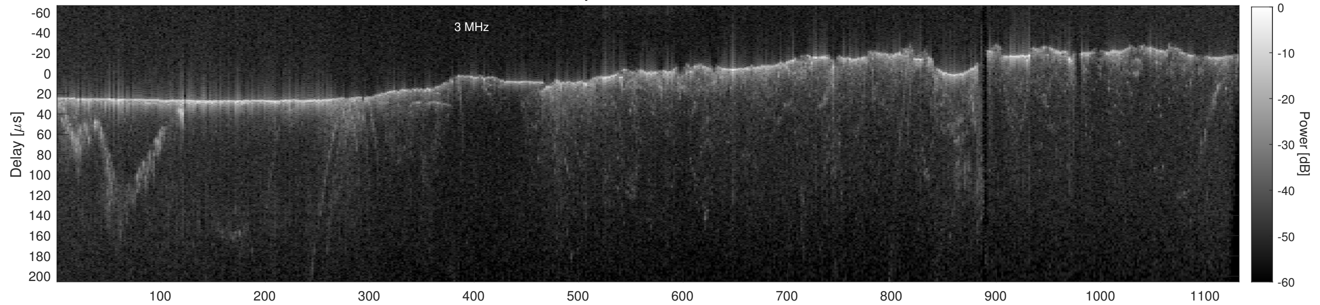
Orbit 21747, Cluttergram
