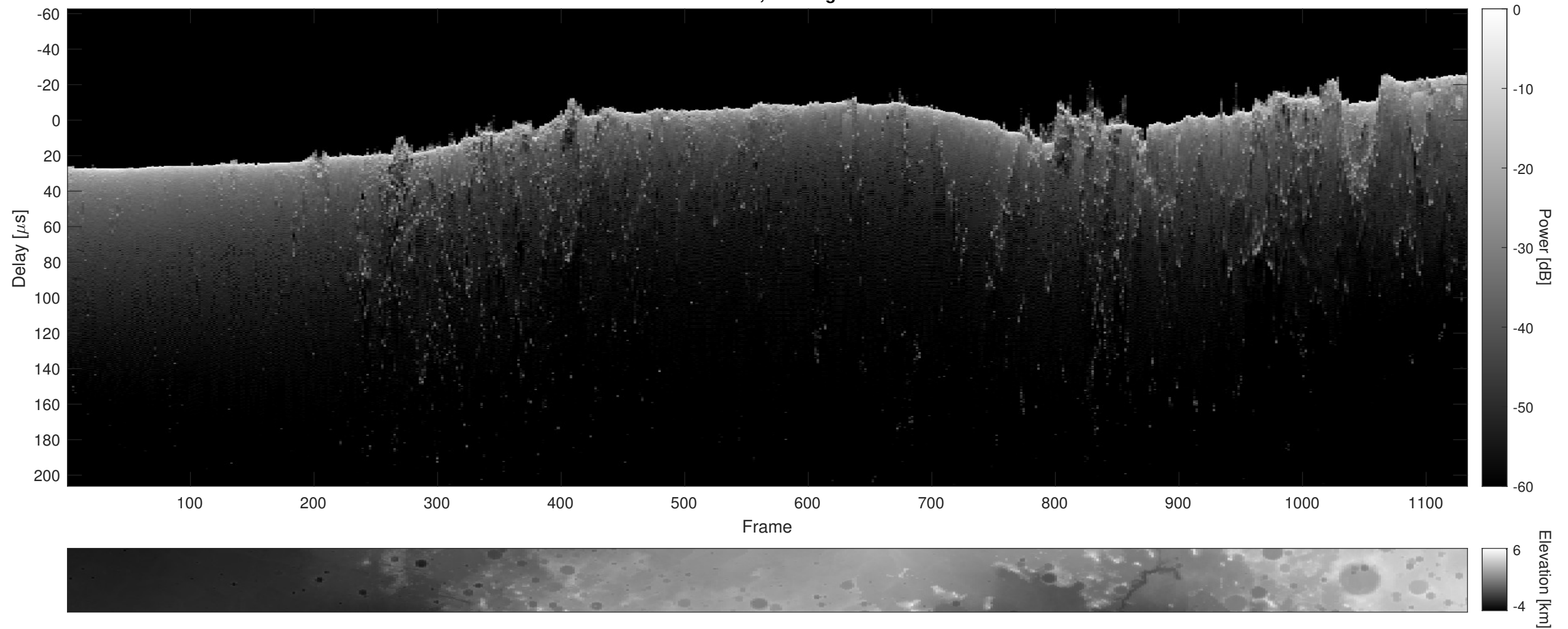
Orbit 21748, Cluttergram
