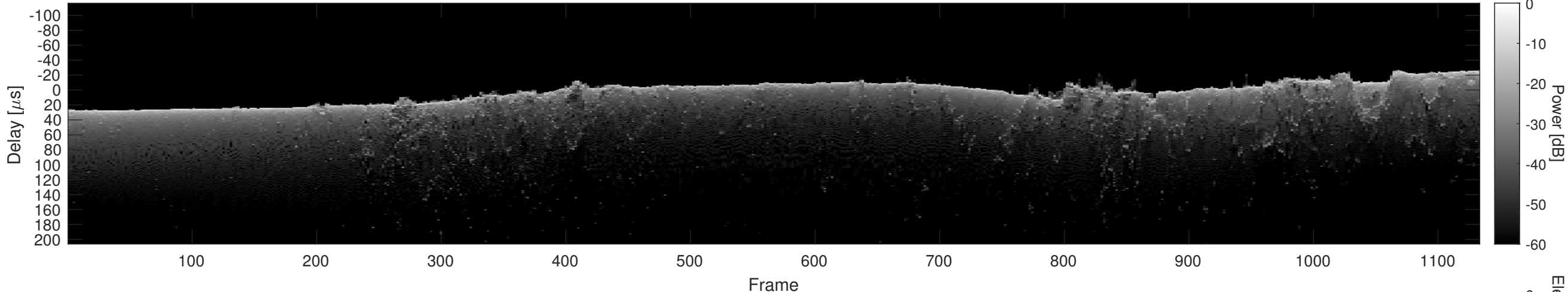
Orbit 21748, Cluttergram
