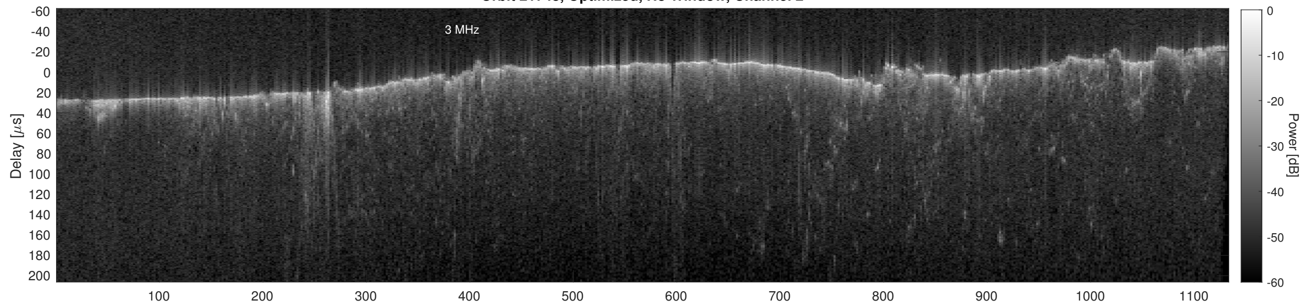
Orbit 21748, Cluttergram
