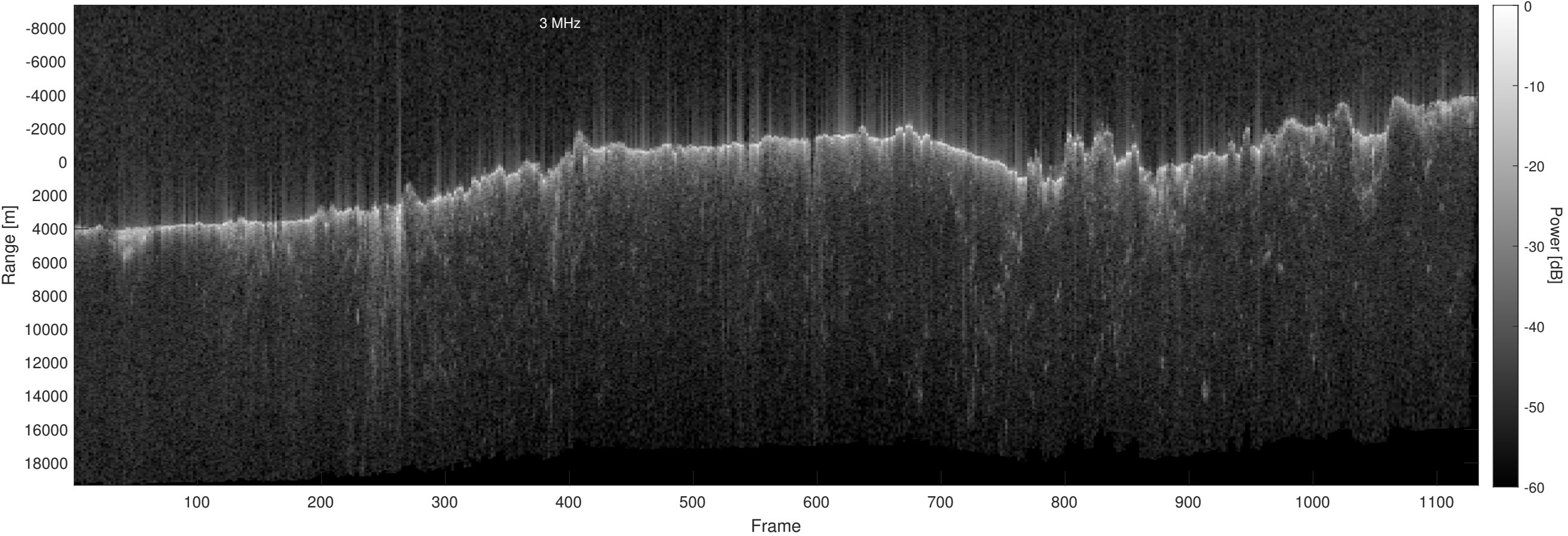
Orbit 21748, Optimized, No Window, Depth-Corrected, Channel 2
