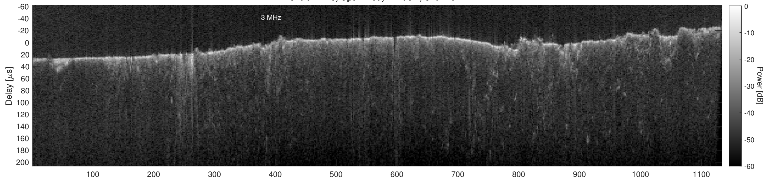
Orbit 21748, Cluttergram
