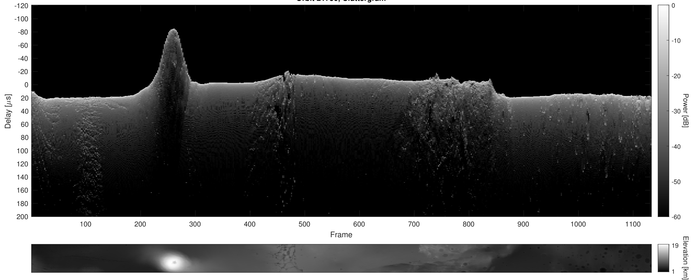
Orbit 21750, Cluttergram
