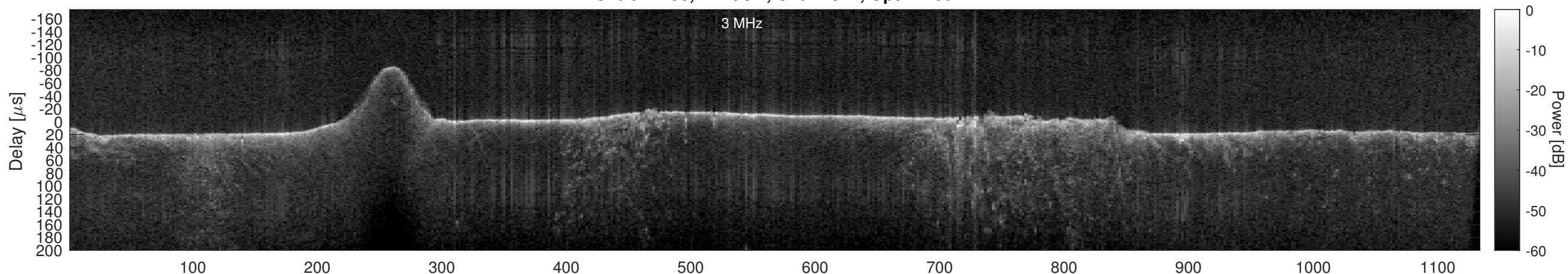
Orbit 21750, Cluttergram
