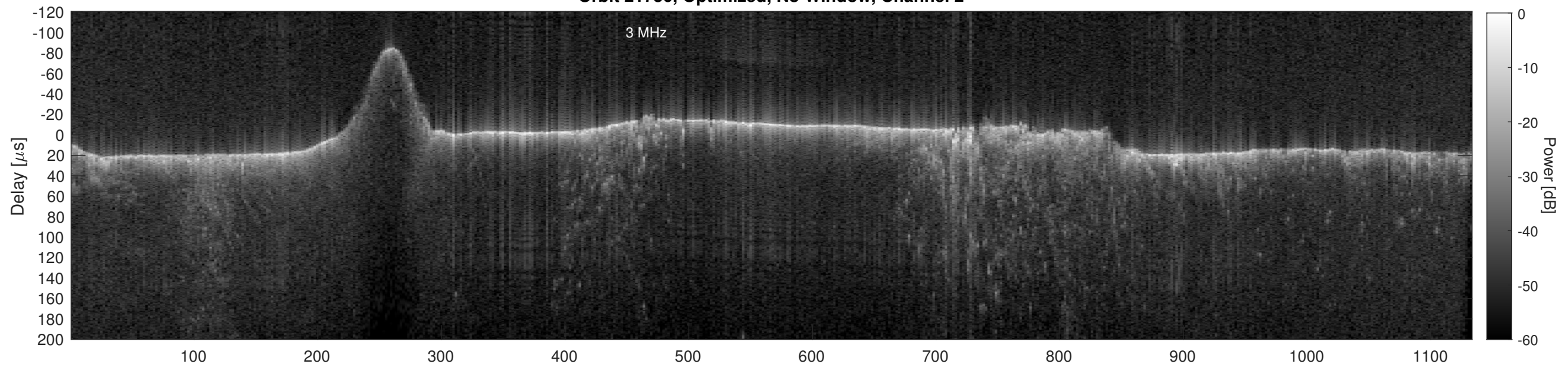
Orbit 21750, Cluttergram
