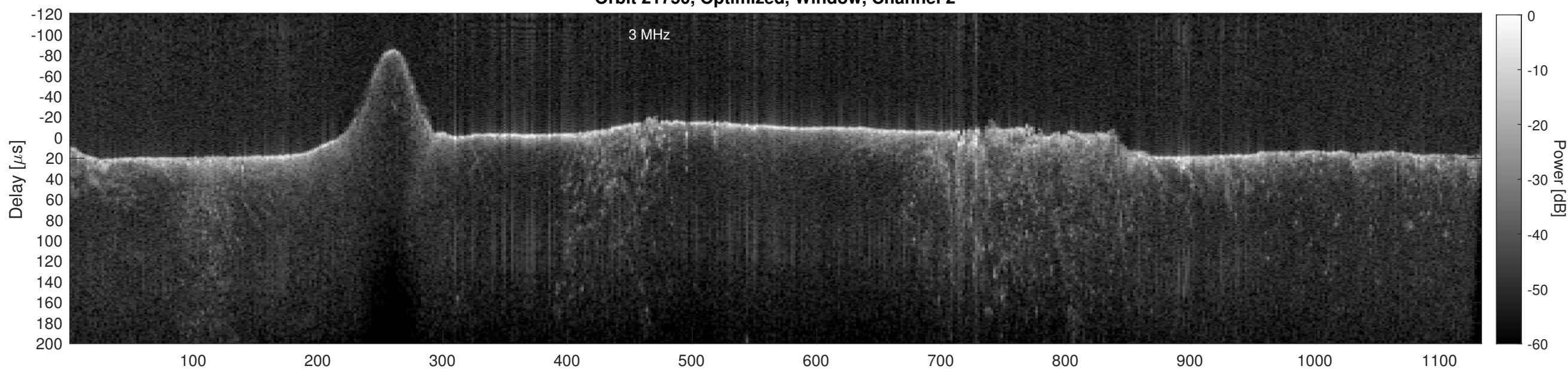
Orbit 21750, Cluttergram
