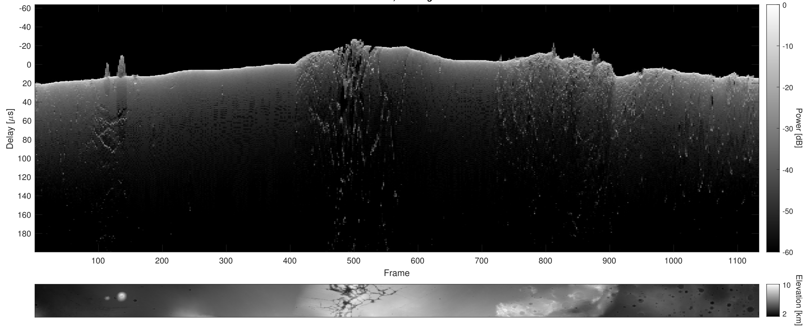
Orbit 21757, Cluttergram
