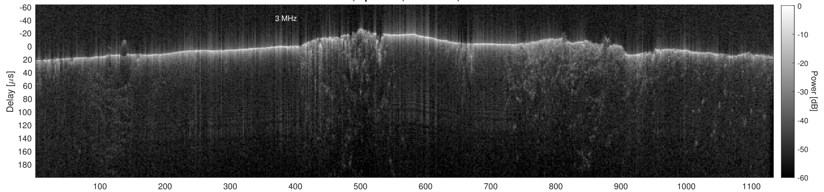
Orbit 21757, Cluttergram
