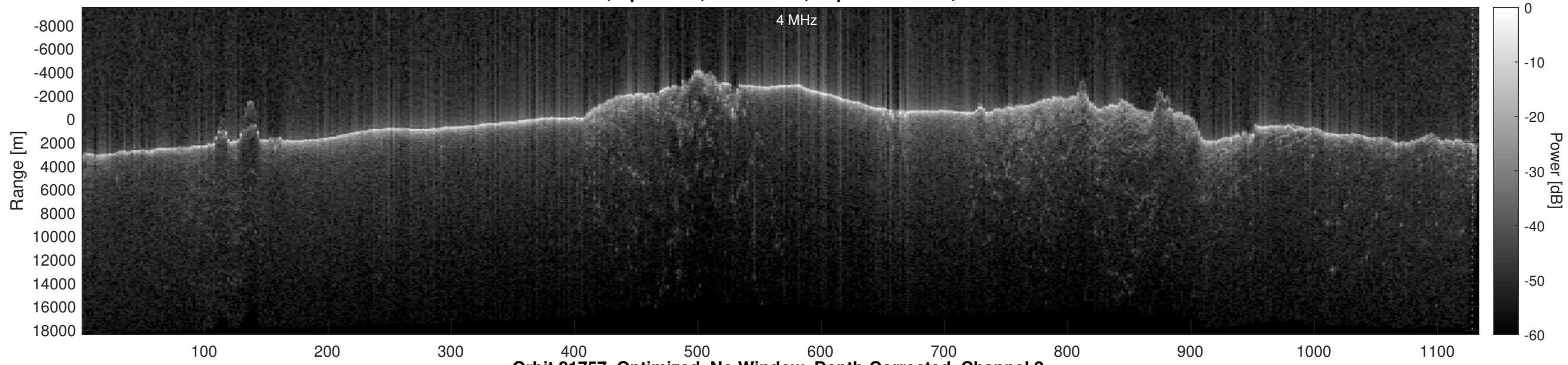
Orbit 21757, Optimized, No Window, Depth-Corrected, Channel 2
