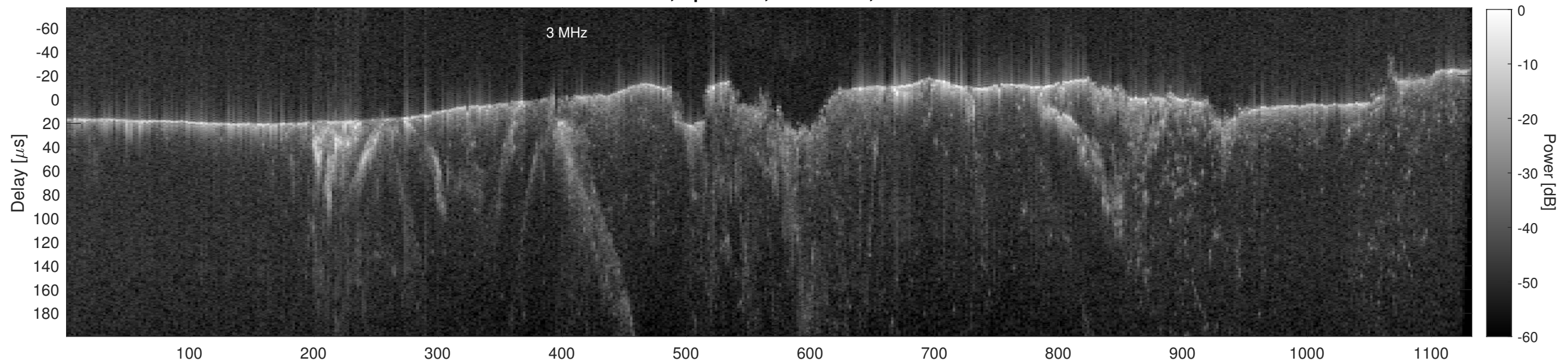
Orbit 21760, Cluttergram
