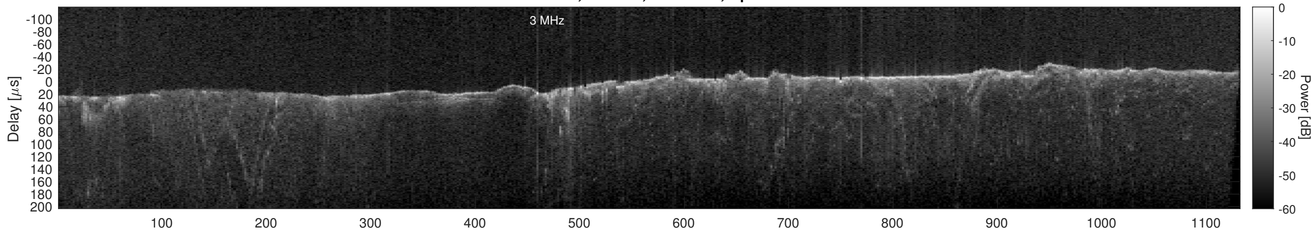
Orbit 21761, Cluttergram
