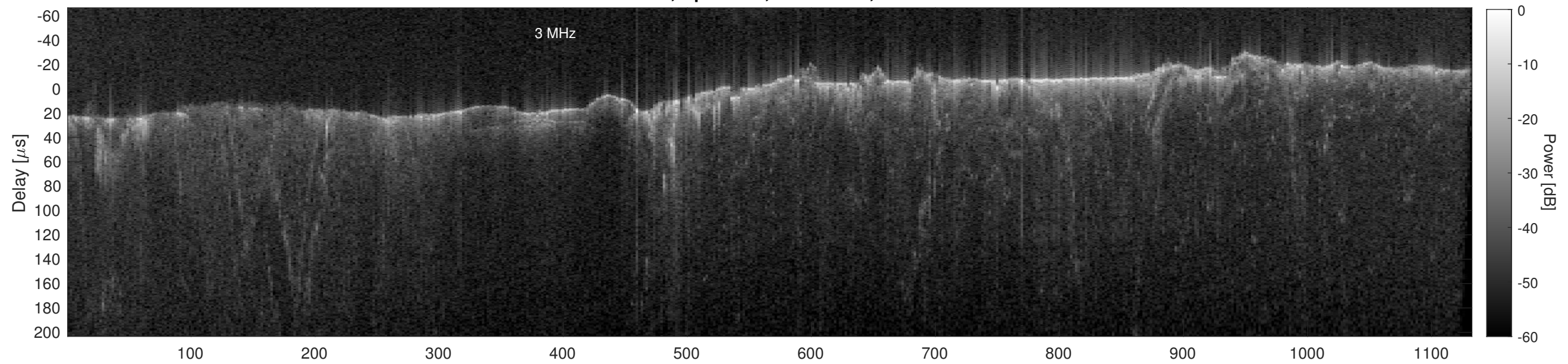
Orbit 21761, Cluttergram
