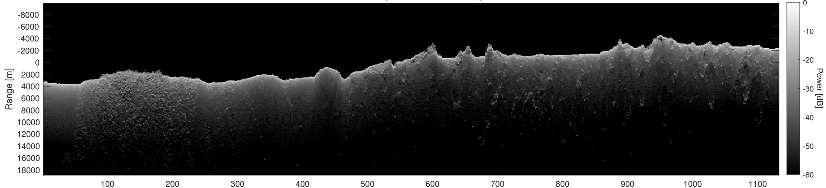
Orbit 21761, Depth-Corrected Cluttergram
