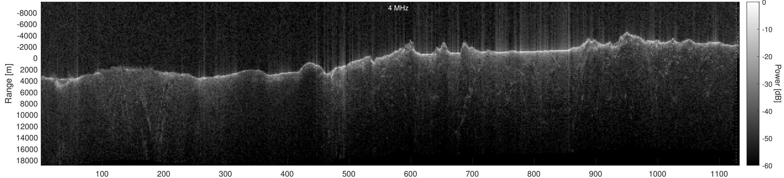
Orbit 21761, Optimized, No Window, Depth-Corrected, Channel 2
