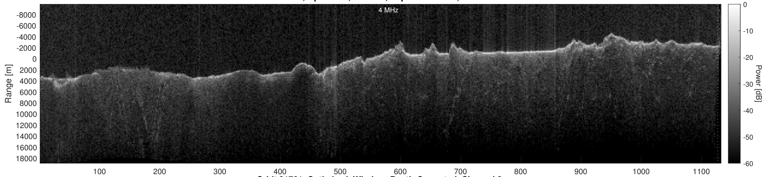
Orbit 21761, Optimized, Window, Depth-Corrected, Channel 2
