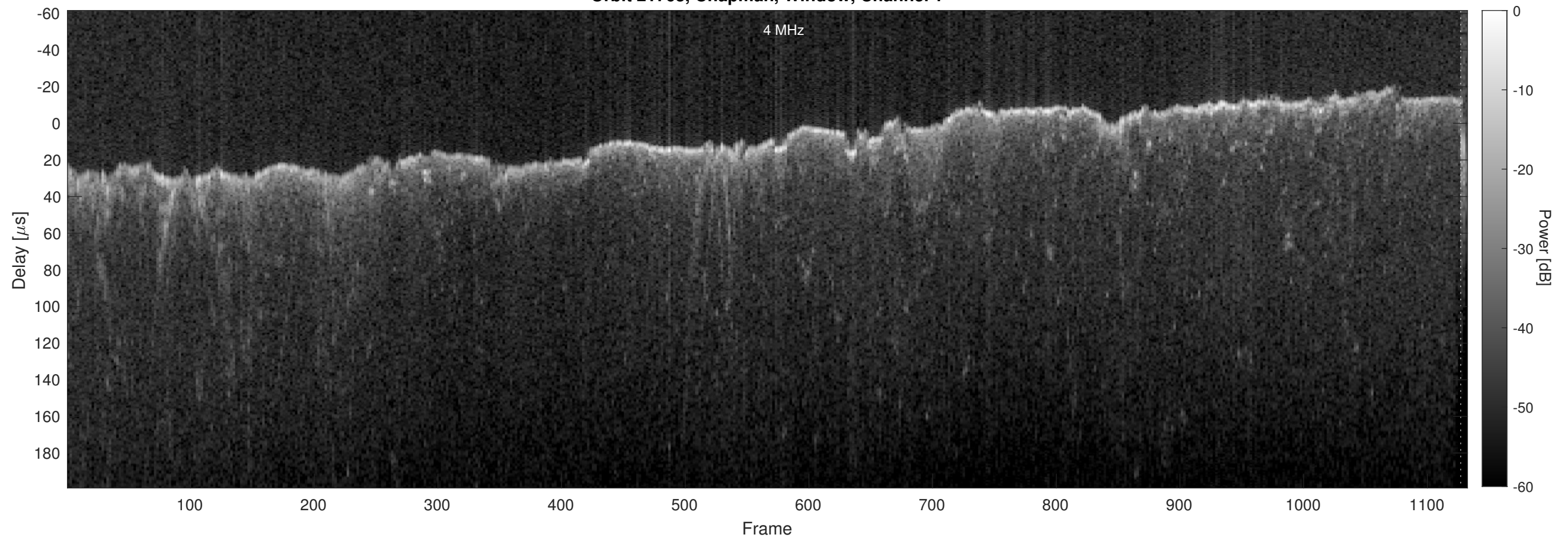
Orbit 21763, Chapman, Window, Channel 2
