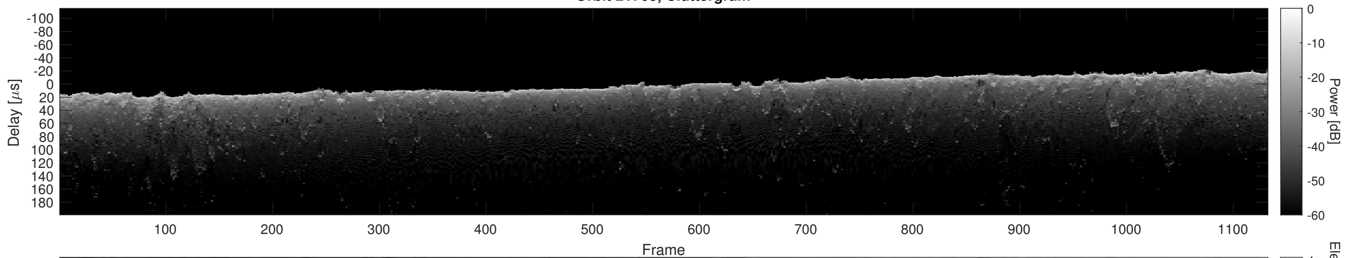
Orbit 21763, Cluttergram
