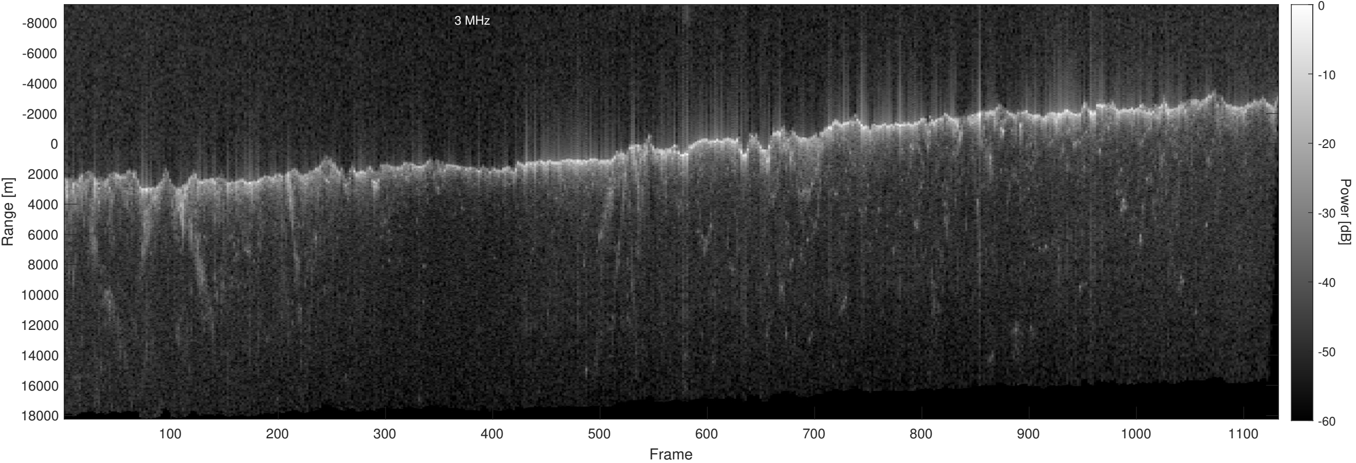
Orbit 21763, Optimized, No Window, Depth-Corrected, Channel 2
