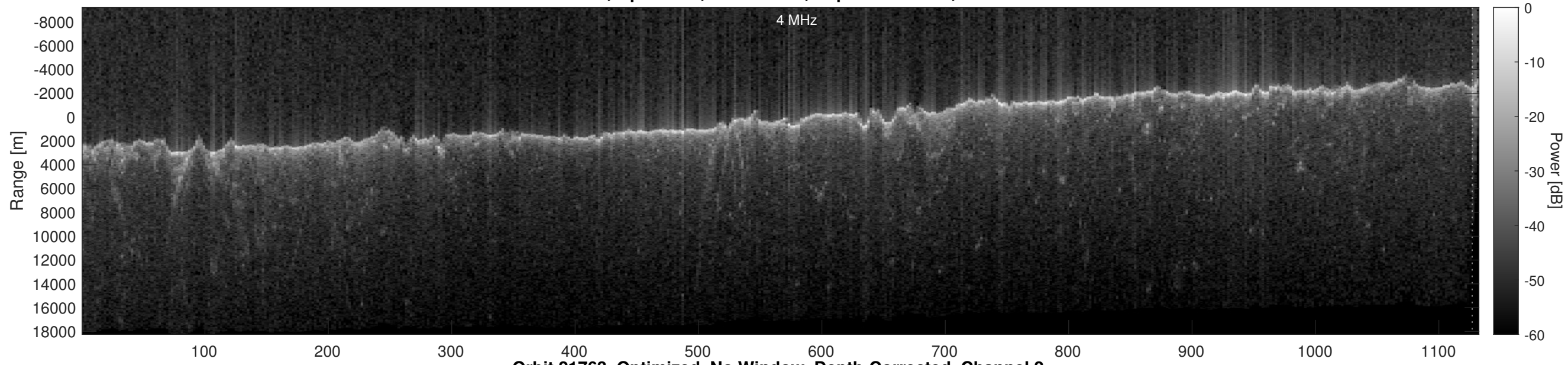
Orbit 21763, Optimized, No Window, Depth-Corrected, Channel 2
