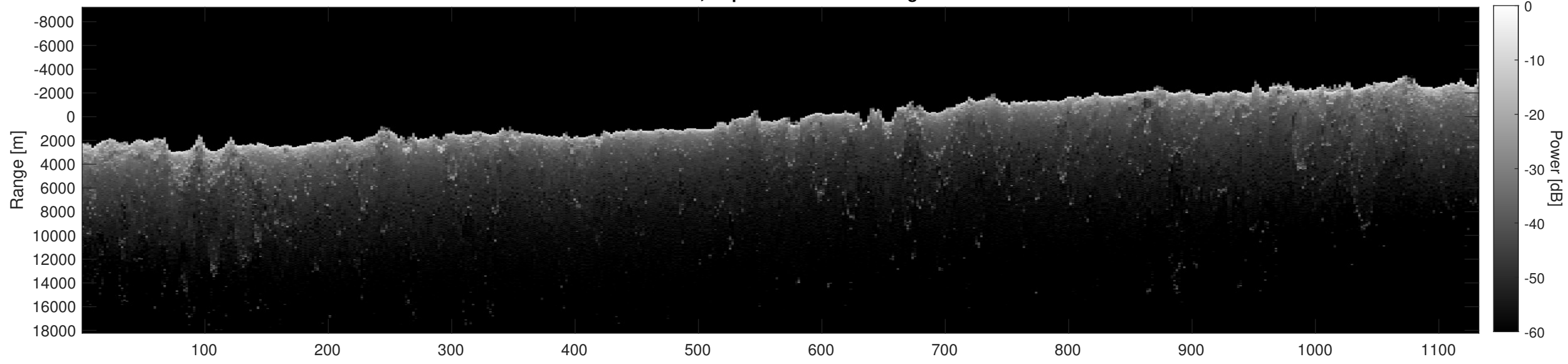
Orbit 21763, Depth-Corrected Cluttergram
