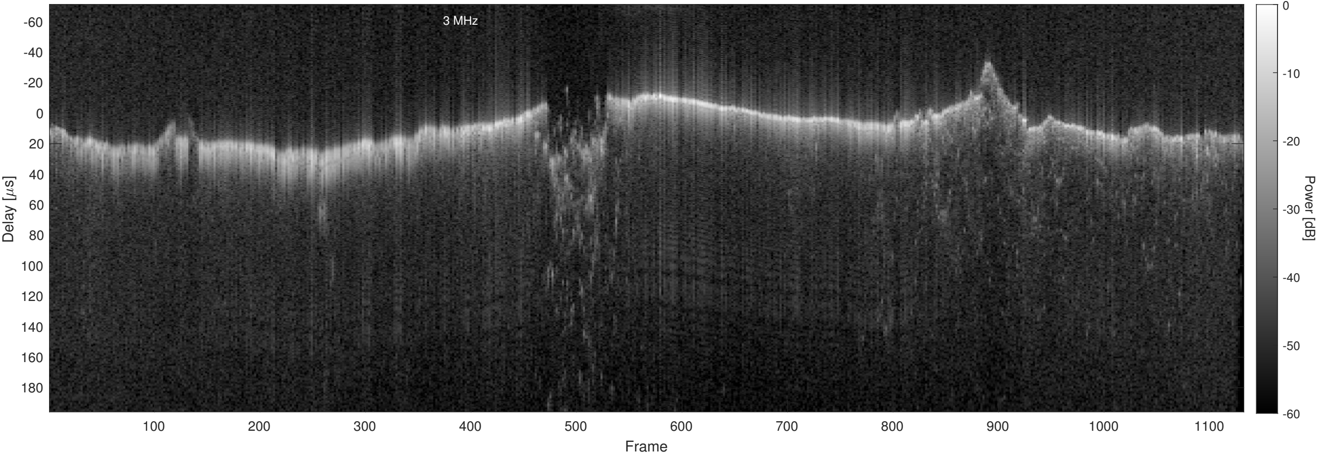
Orbit 21764, Chapman, No Window, Channel 2
