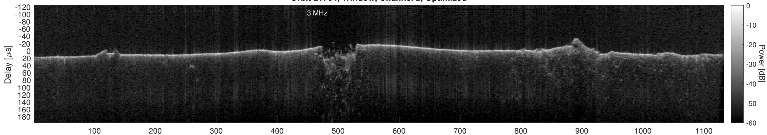
Orbit 21764, Cluttergram
