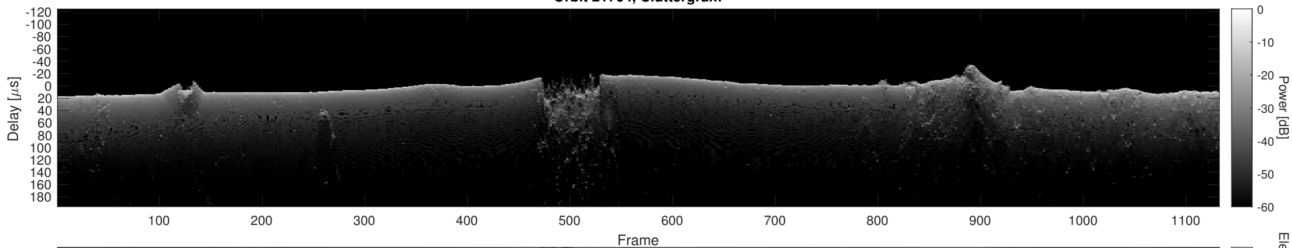
Orbit 21764, Cluttergram
